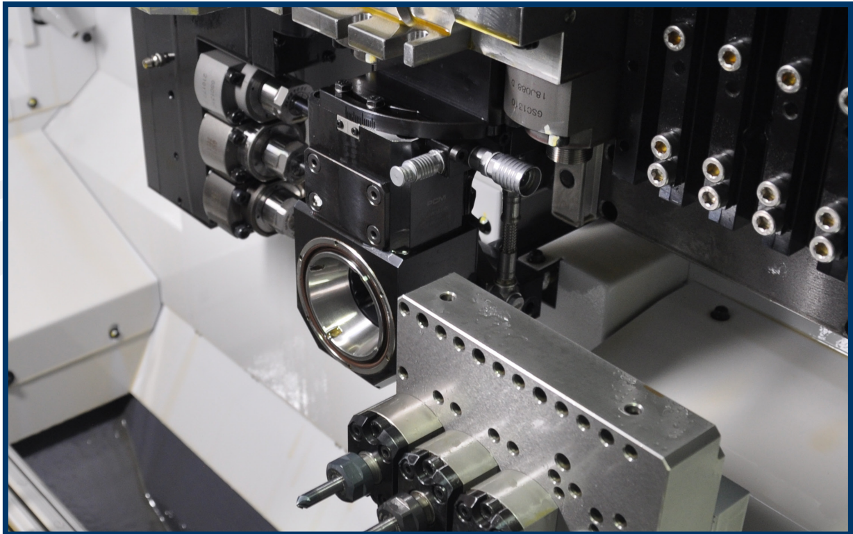
Thread whirling toolholder GSW161 mounted on a CITIZEN L20-2M12 machine
